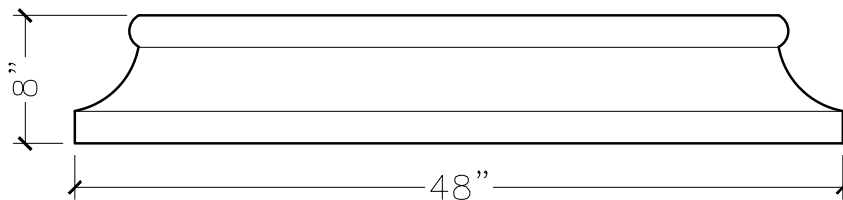
FRONT VIEW
