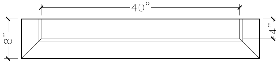
TOP VIEW
