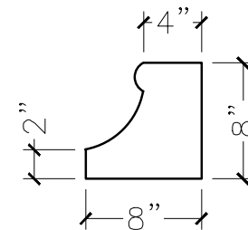
SECTION VIEW
