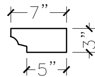
SECTION VIEW
