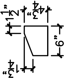
SECTION VIEW
