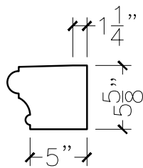
SECTION VIEW
