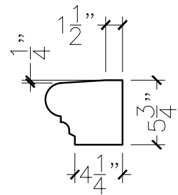
SECTION VIEW
