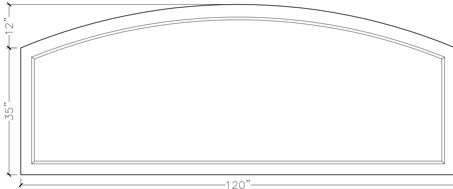
FRONT VIEW
