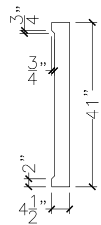
SECTION VIEW
