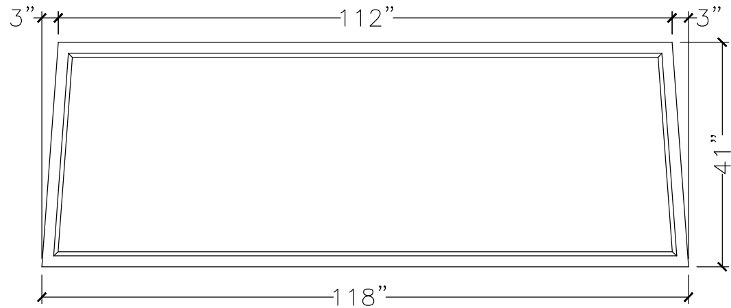
FRONT VIEW
