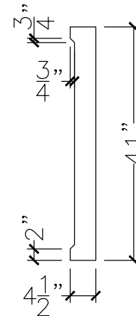
SECTION VIEW
