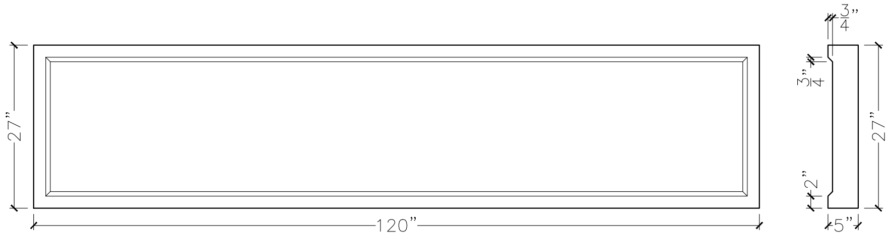
FRONT VIEW
