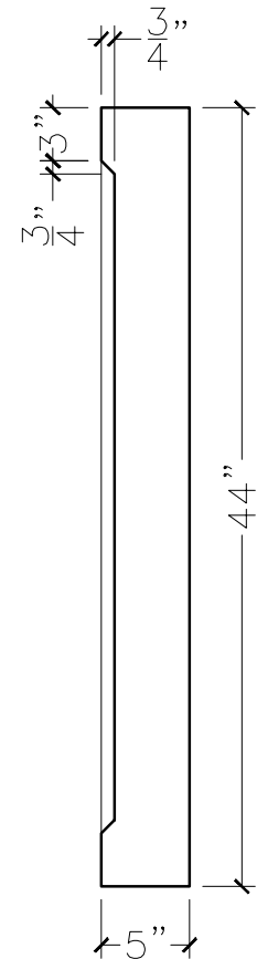
SECTION VIEW
