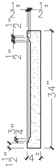
SECTION VIEW
