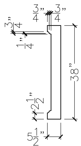
SECTION VIEW
