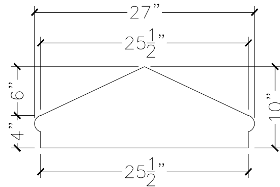
SECTION VIEW
