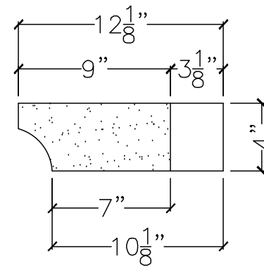
SECTION VIEW
