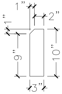
SECTION VIEW
