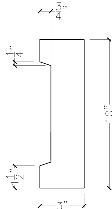
SECTION VIEW
